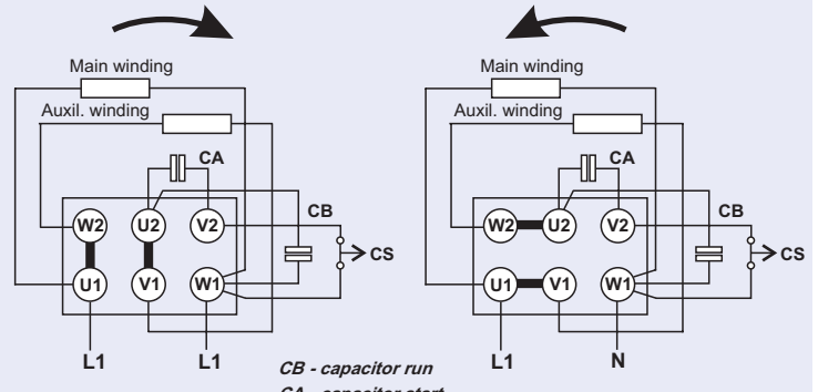
2. With capacitors start / run
