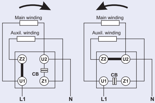
CB - capacitor run
